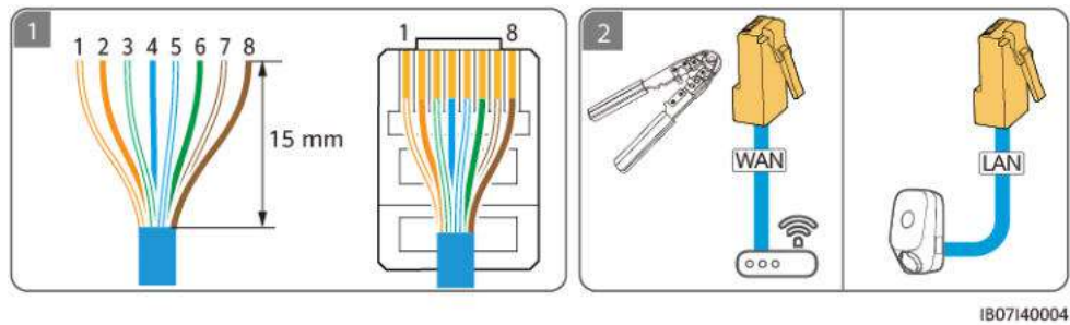
Figure 5-18 Câble de communication FE
