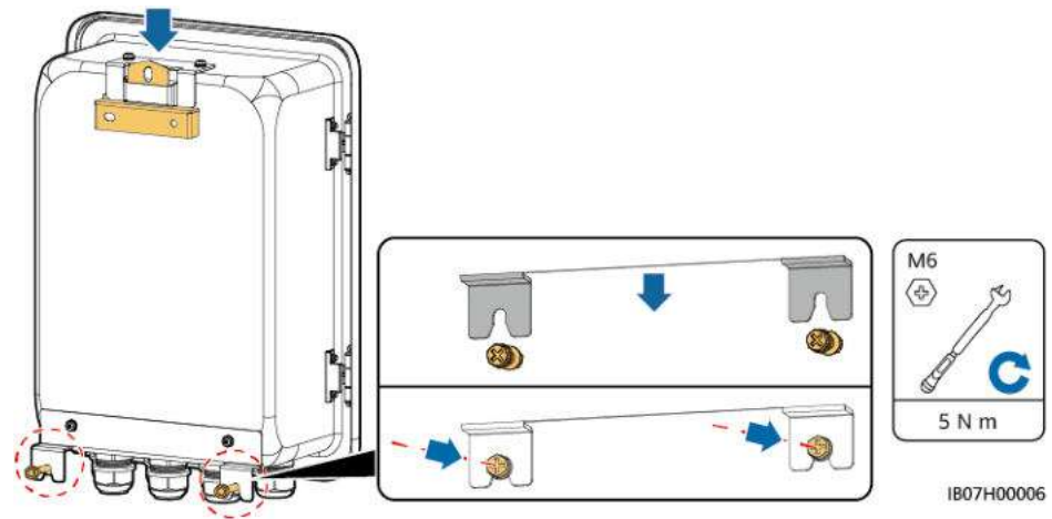
Figure 4-10 Installation du SmartGuard
