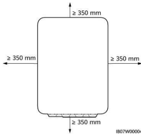
Figure 4-2 Distances
