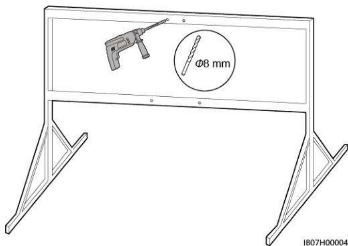
Figure 4-8 Forage des trous
