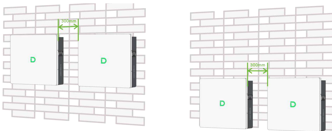
Installation murale
